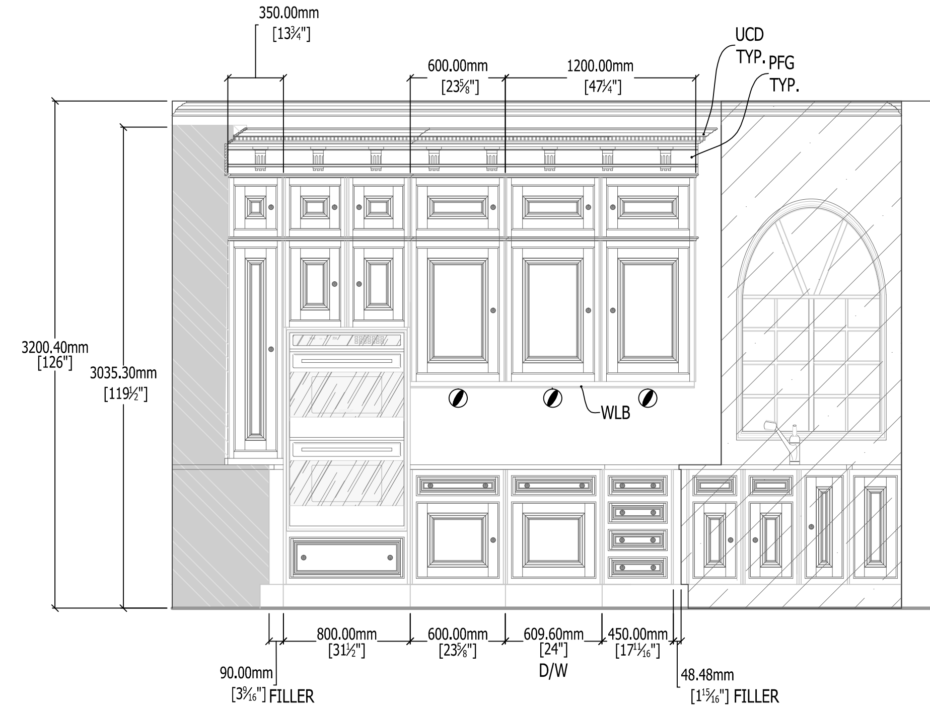
ELEVATION "B"
