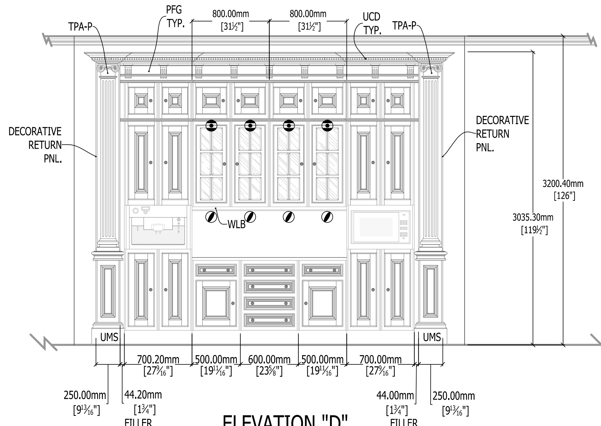
ELEVATION "D"
